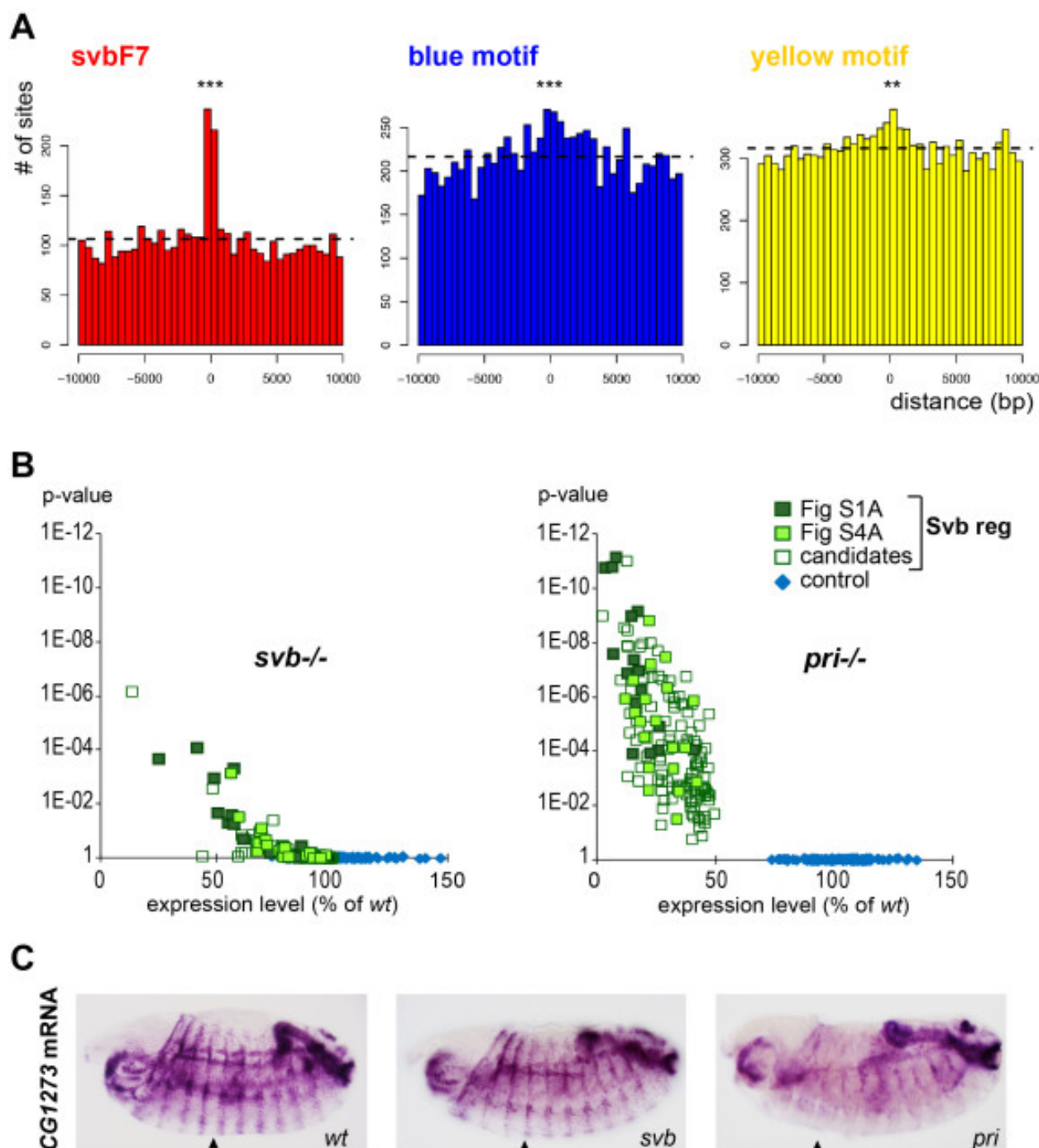
Figure 6 Genome-wide profiling of embryonic genes regulated by Svb. (a) Cross-correlation between conserved svbF7, blue or yellow motif instances and Svb ChIP-seq peaks throughout the whole genome. Plots show the number of motifs found in a 10 kb window on each side of the center of peaks. The P -value for correlation (Chi2 test) is <1E-46 , <1E-9 and <1E-2 for svbF7, blue and yellow motifs, respectively. *** indicates a P -value < 0.001 , ** < 0.01 . Dashed line shows the average number of sites across the region. (b) Modifications in mRNA levels as measured by microarrays between wild-type (wt) and svb (left) or pri (right) embryos in Svb-regulated (green) and control (blue) sets of genes. Dark green dots represent known Svb targets (Figure S1A in Additional file 1), light green novel target genes as validated by in situ hybridization (Figure S4 in Additional file 1) and open dots additional candidates. (c) Whole mount in situ hybridization of CG1273, a Svb downstream target identified from microarray profiling, down-regulated in trichome cells (arrowheads show a row of ventral trichome cells) of svb mutants and showing further reduced expression in pri mutant embryos.
