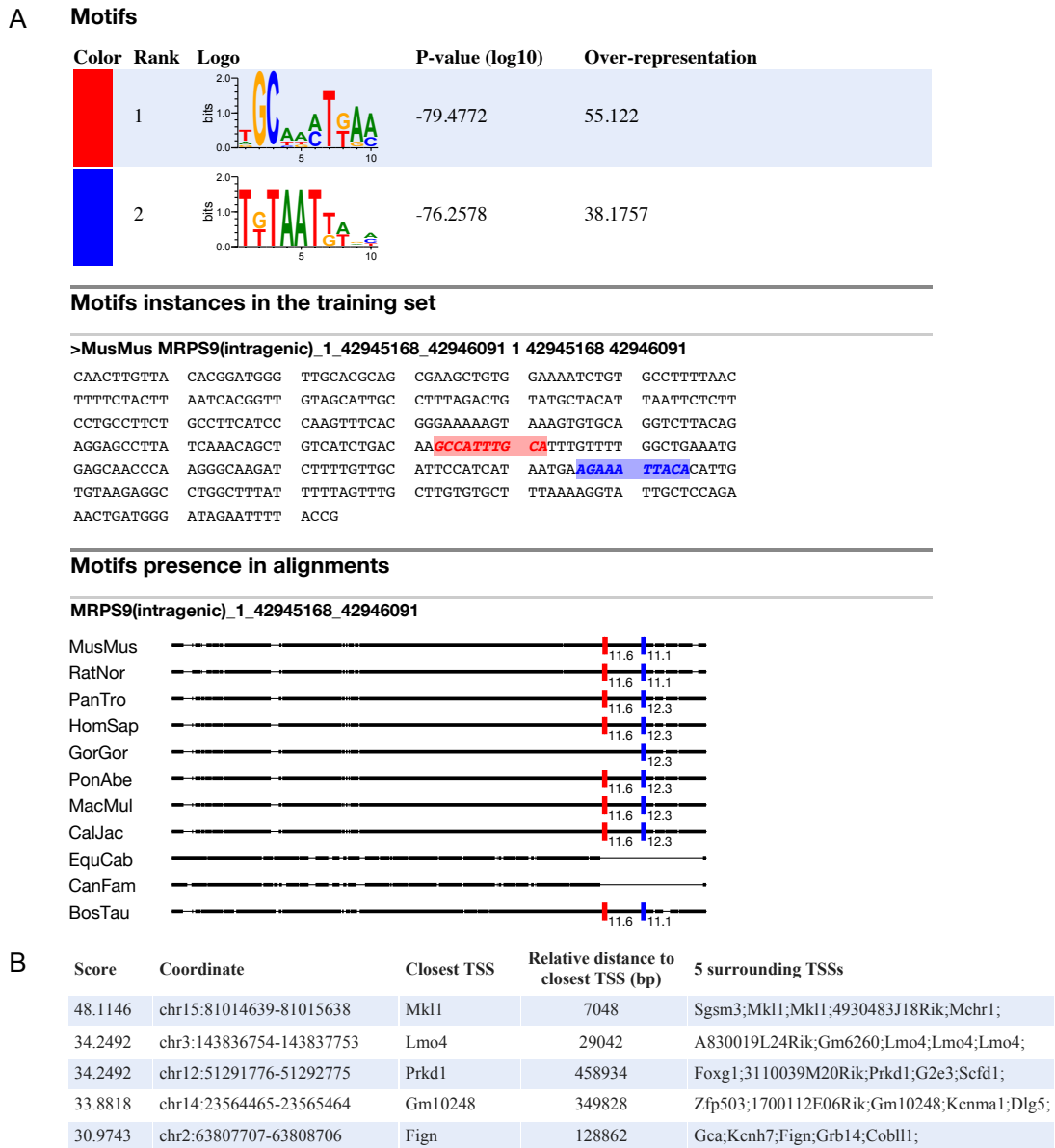
Figure 7. Web based interface : output web page. Example of an output web page for Imogene powered by the mobyle bioinformatics framework. A. Result page for the Genmot mode. Two motifs were generated from the neural tube full training set (default is 5), using the same parameters as in Figure 3. Results are shown for the training set sequence MRPS9(intragenic). For display purposes, the beginning of the sequence, which contains no instances for the motifs, was cut in the middle panel. In the alignments, thick lines correspond to sequences and thin lines to gaps. B. Result page for the Scangen mode. The two generated motifs were used to score putative regulatory sequences of 1kb in the mouse genome at optimal threshold S_s = 10 . The 5 best ranking sequences are shown (default is 200).
