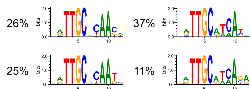
Pairwise model
